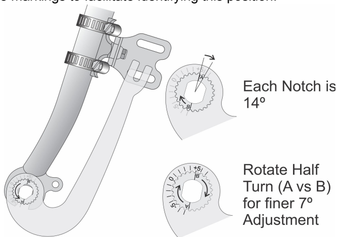
Figure 5: Orient the insert to line up with axle flats. Laser markings help facilitate and recall alignment
