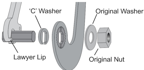
Figure 7: Recommended order of axle hardware
