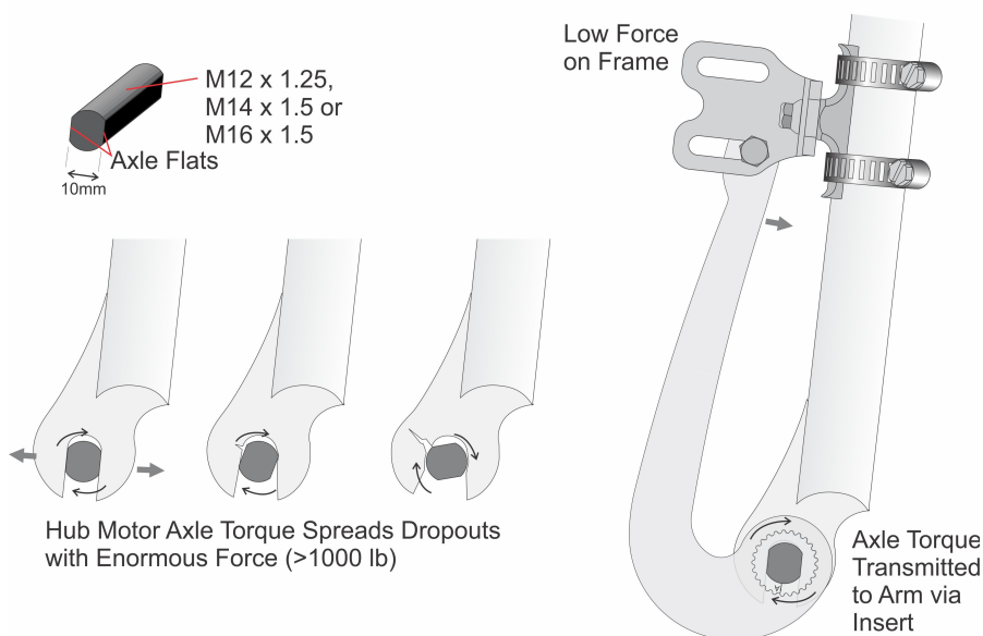
Figure 2: Illustration of axle spinout and effects of torque arm
