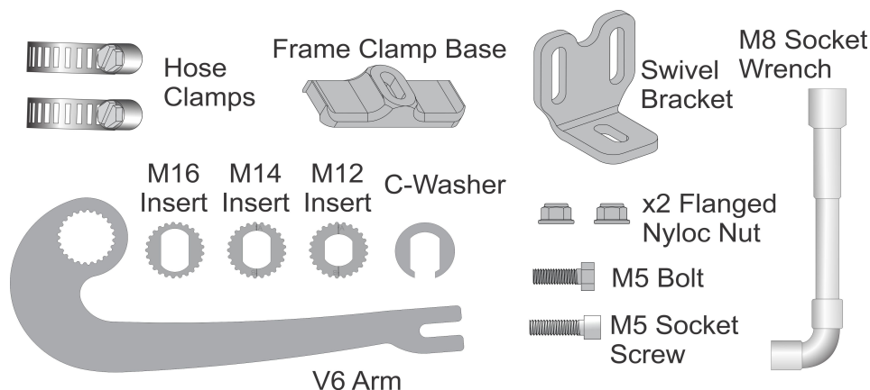
Figure 1: Parts included in V6 Torque Arm package
