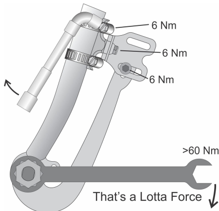
Figure 8: Tightening torques
