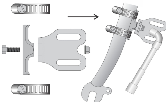
Figure 4: Frame Clamp loosely in place
