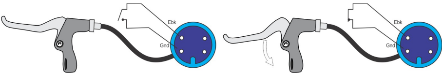
Figure 7: Most Ebrakes are switches that connect the ebrake signal line to ground when the brake lever is pressed. Pinout shown is from male connector perspective.
