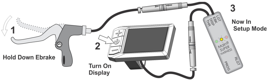
Figure 14: Accessing the setup mode. Yellow LED will strobe.
