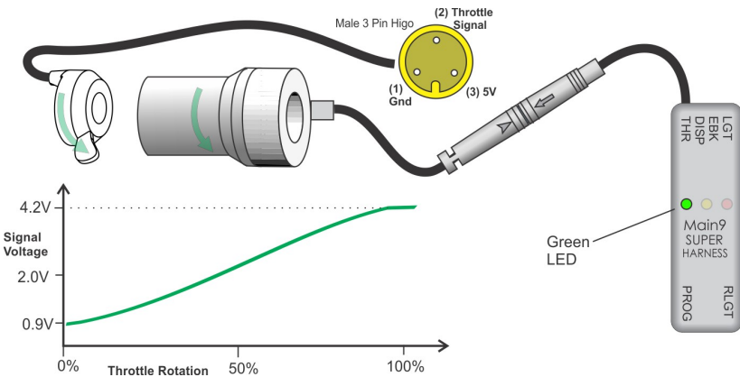
Figure 5: Signal output of a typical throttle. Green LED increases in brightness with throttle position. Pinout shows male throttle side Higo connector.
