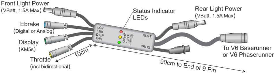
Figure 2: Superharness contains active circuitry
