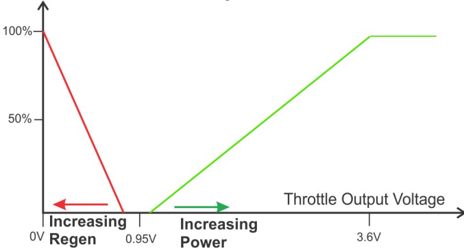
Figure 4: Single throttle output voltage of Superharness controls both power and regenerative braking in Phaserunner/Baserunner controllers.
