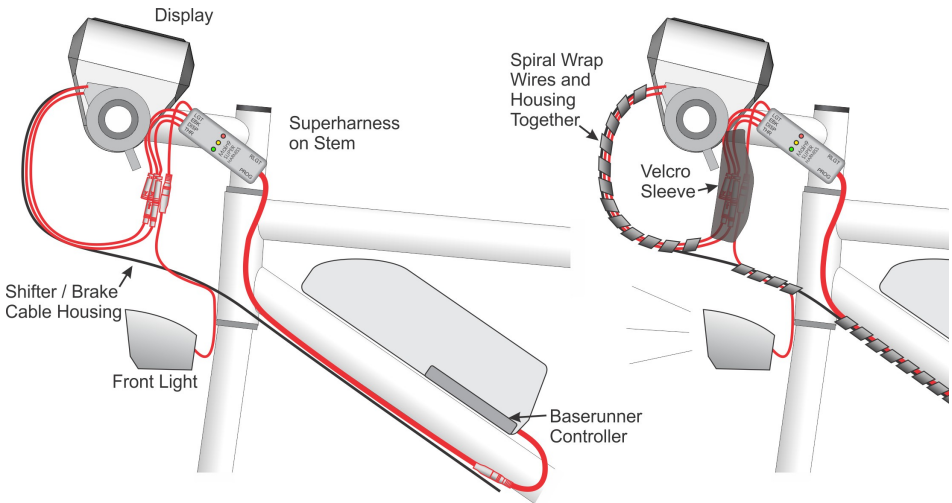
Figure 13: Recommended wire management strategy that eliminates need to bundle excess cable. Wires (shown red) should follow existing shifter/brake cable housings (black). Multiple short pieces of spiral wrap is easier to handle than one long length.
