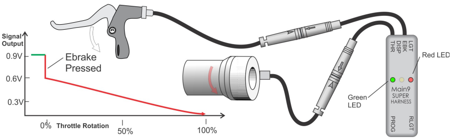
Figure 8: When throttle is engaged at the same time as digital brake cutoff, it controls the regen intensity by modulating output down to 0.0V
