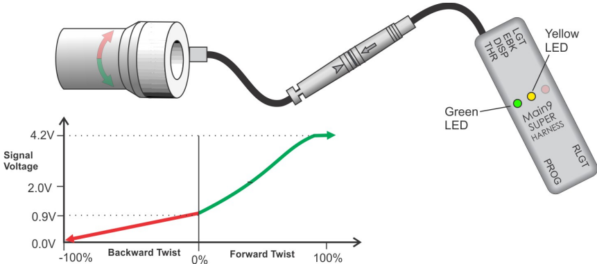
Figure 6: Bidirectional throttles have mid point, allowing both forward and backward twisting. In neutral position signal should sit at ~0.9V. Two-way throttles with 2.5V midpoint are not compatible.
