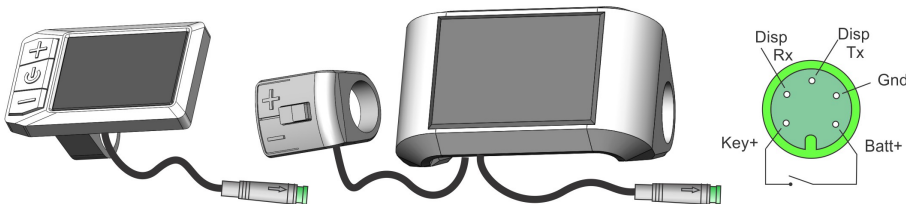
Figure 10: Small displays are available with integrated buttons (left), while larger central displays have separate handlebar switch. Male side display pinout shown. System only powers on when Key+ is switched to Batt+.
