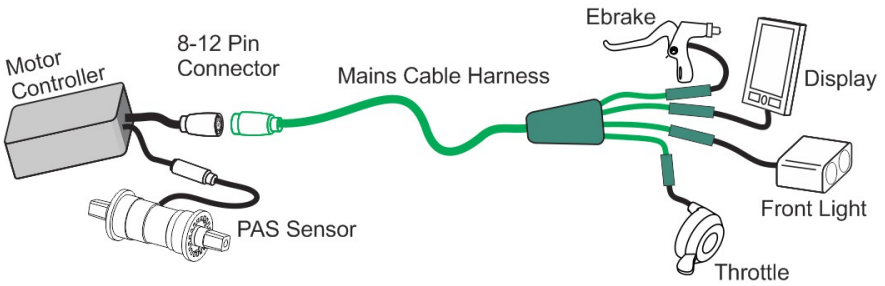
Figure 1: Example of a Mains Harness (Green)
