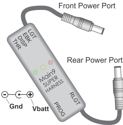
Figure 11: 5.5 x 2.1mm jacks provide convenient access to DC battery power for accessories.
