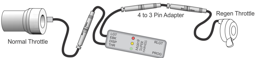
Figure 18: A regular throttle may be used as proportional regen control
