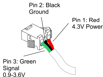
Figure 4: Controller Throttle Pinout
