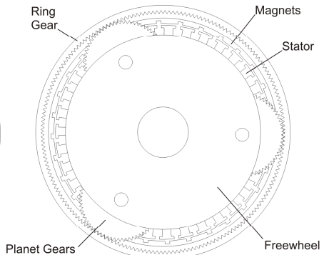
Geared Hub Motor
