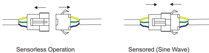
Figure 6: Internal Hall Plug. Inside controller hall wires can be connected or unplugged to change between sensed and sensorless operation
