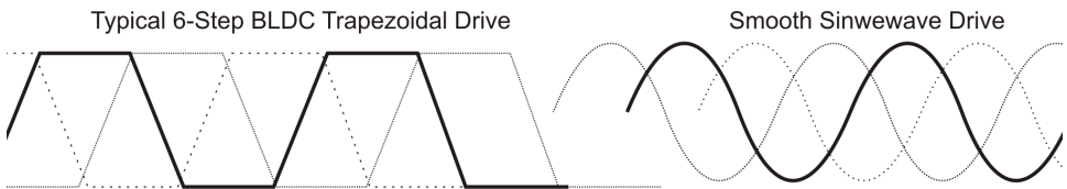
Figure 9: Illustration of Voltage Waveform of Trapezoidal vs Sine Wave Outputs
