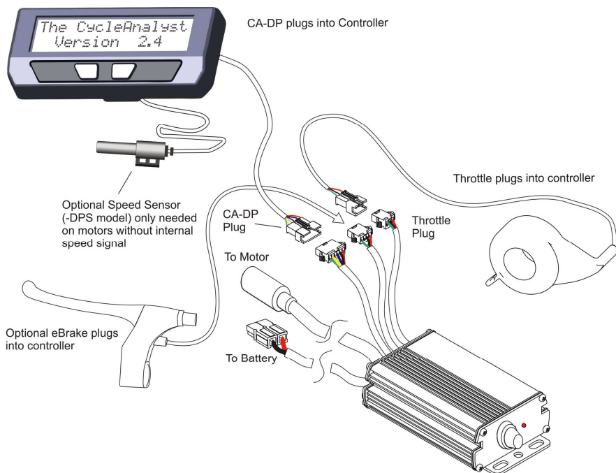
Figure 7: CA V2 Hookup. Throttle and eBrake Plug into Controller (motor and battery not Shown)
